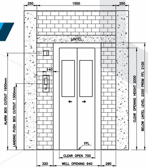
LIFT FRONT ENTRANCE WALL
