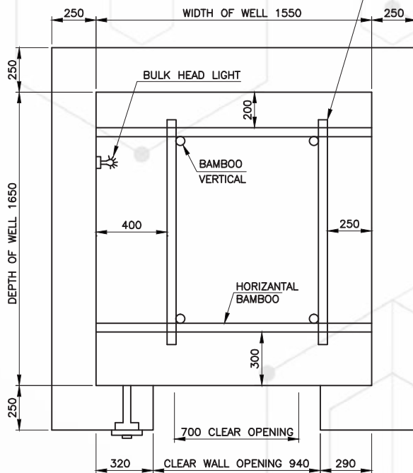
SCAFFOLDING DETAIL
