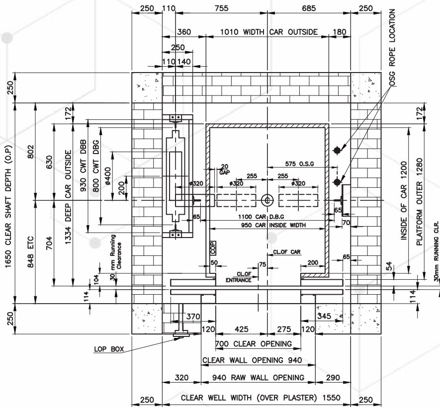
LIFT WELL & CAR PLAN
